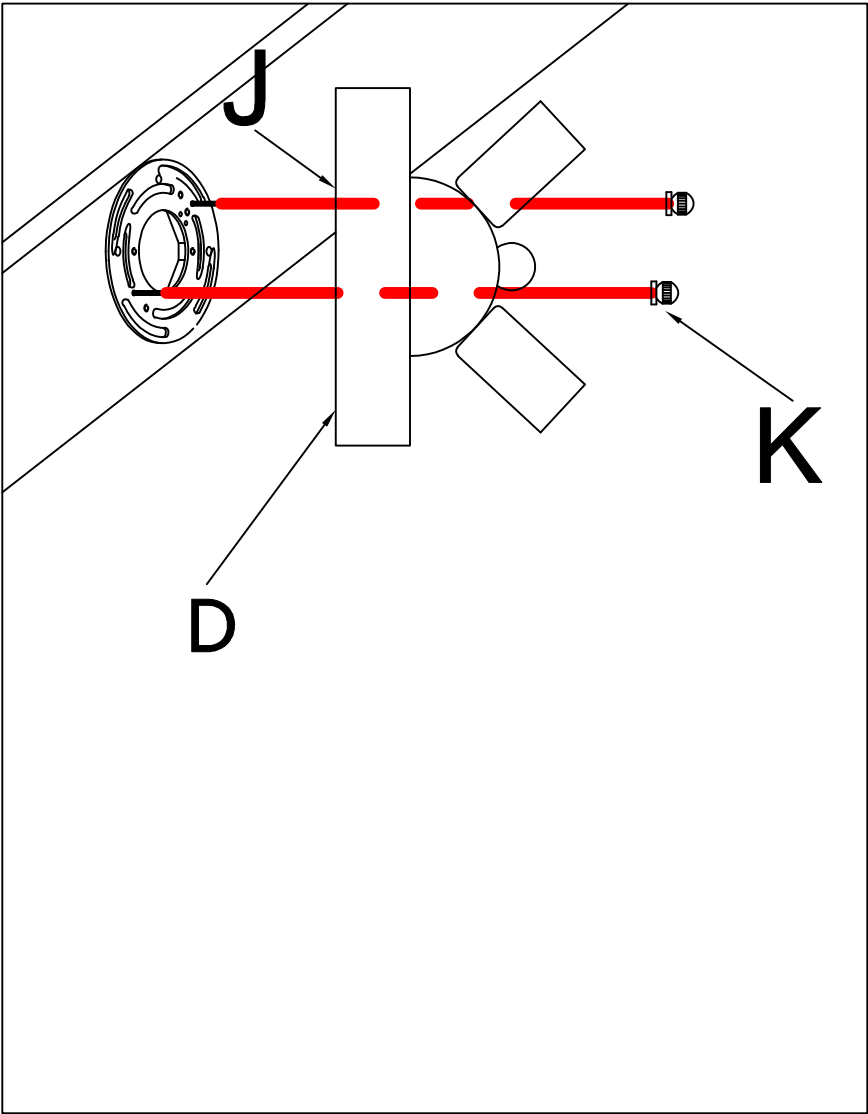
STEP 2: Fix the lamp body(D)on the hanging board,then lock the nut(K)closely.
