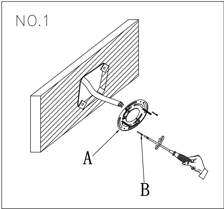
STEP 1: Fix bracket (A) by monting screws (B)
