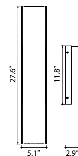
EW10503/LED-28/AL EW10504/LED-28/BX
