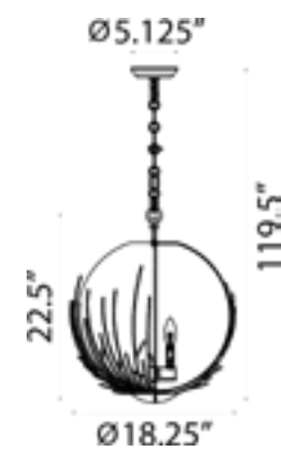
P30061/5/AGB P30059/5/SBB
